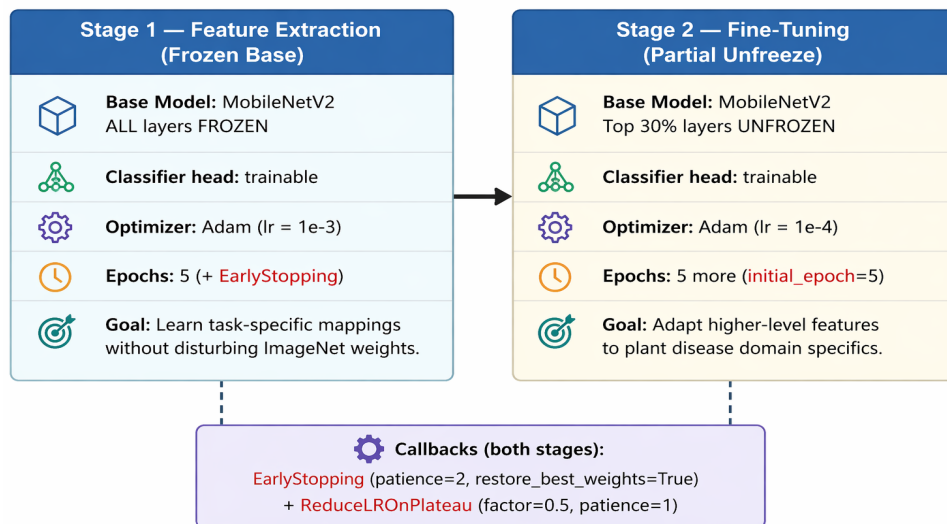
Figure 1: Two-Stage Training Strategy
