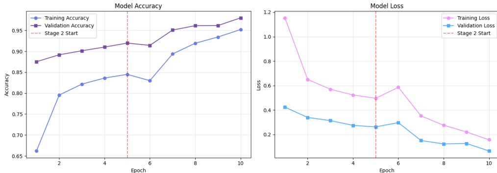
Figure 2: Training and Validation Accuracy and Loss Curves
